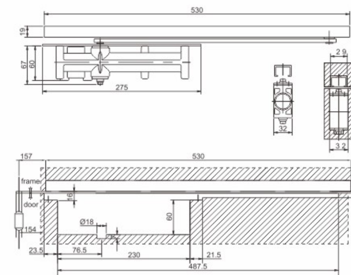
103 104 Dimensioned Drawing
