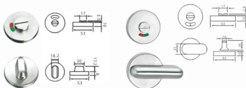
BK1BK3 SS AVAILABLE : BLACK
