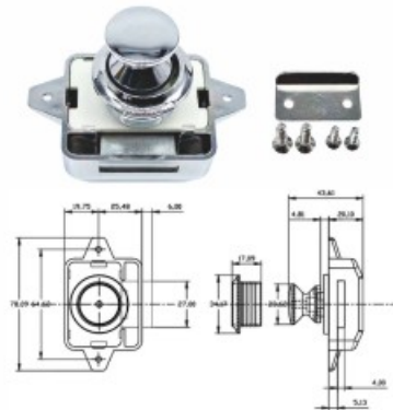
RV PUSH BUTTON DRAWER LOCK
