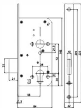
7210-55D SS (BLACK)
